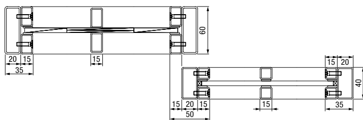
Horizontal view double-leaf steel loft door with side element
