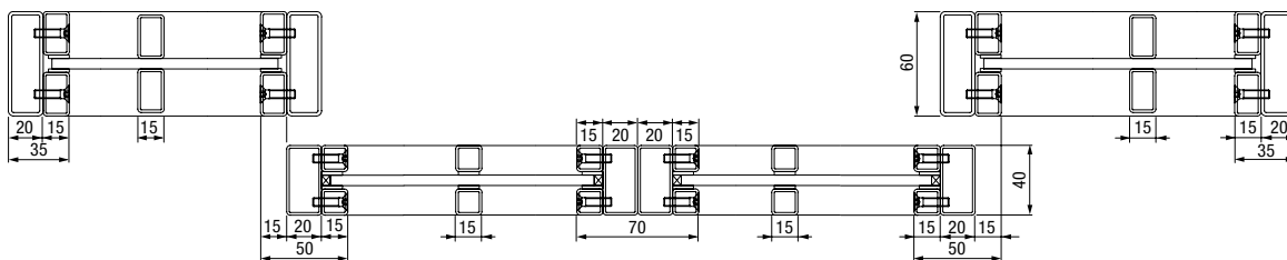
Horizontal view, double-leaf steel loft door with side elements
