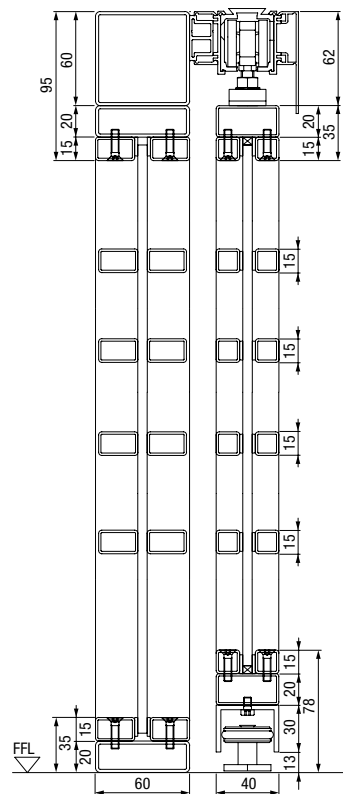
Vertical view double-leaf steel loft door with side element
