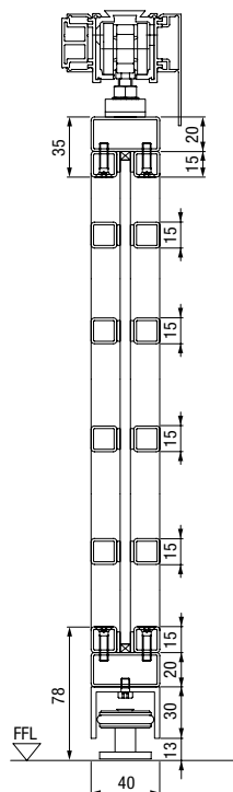
Vertical view single-leaf steel loft door
