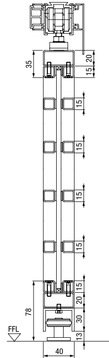
Vertical view double-leaf steel loft door
