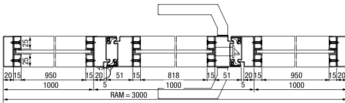
Horizontal view, single-leaf steel loft door with side elements
