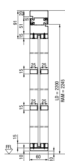
Vertical view single-leaf steel loft door
