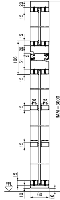
Vertical view single-leaf steel loft door with transom light
