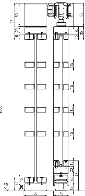
Vertical view double-leaf steel loft door with side elements
