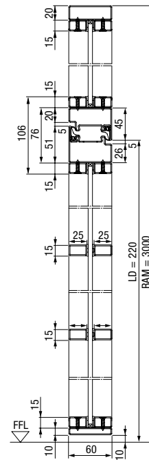
Vertical view double-leaf steel loft door with transom light
