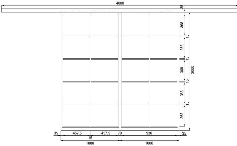
Double-leaf steel loft door
