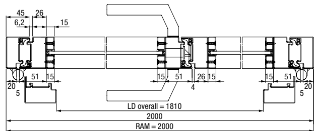
Horizontal view double-leaf steel loft door
