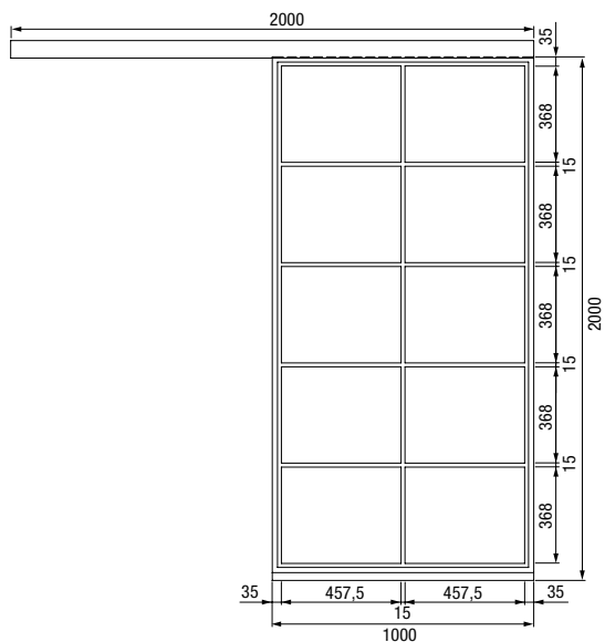
Single-leaf steel loft door
