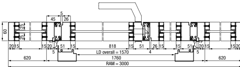
Horizontal view, double-leaf steel loft door with side elements
